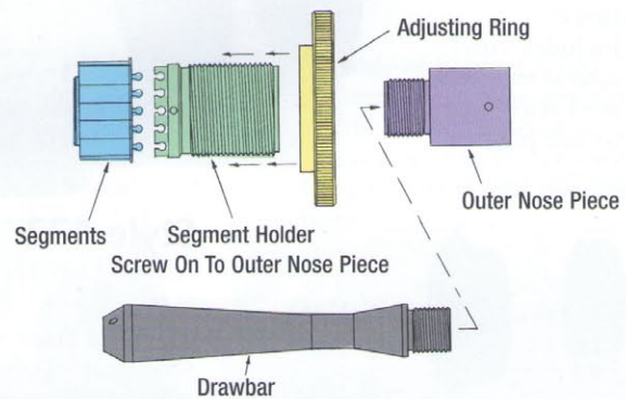
Typical Configuration of 3 1/2", 4", 4 1/2", 5" or 6" Expansion Unit Assembly
