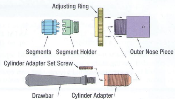
Typical Configuration of 2 1/2", 3" or 3" x 2 1/2" Expansion Unit Assembly
