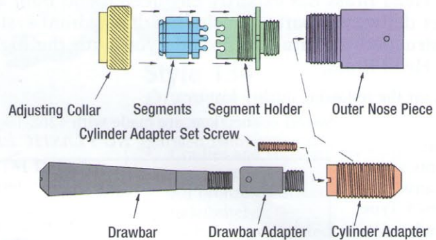
Typical Configuration of 1", 1 1/2", 1 3/4" or 2" Expansion Unit Assembly
